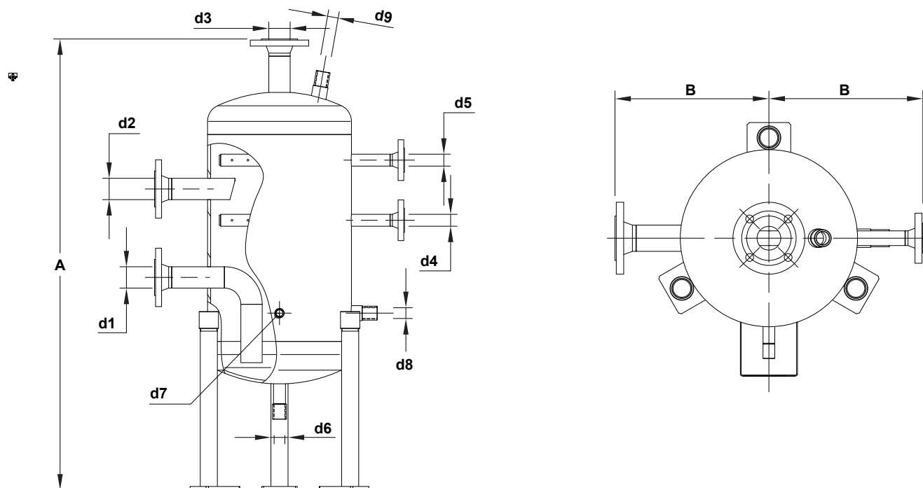
DIMENSIONS (mm) *
